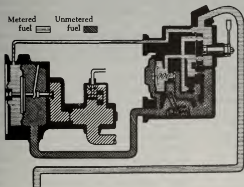
FIGURE 3-29. Power enrichment system.
